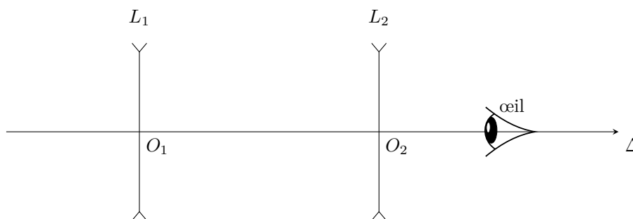
FIGURE 1.2 – Doublet de lentilles.
